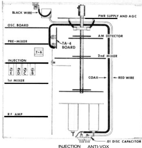
TA4 CIRCUIT BOARD INSTALLATION DIAGRAM (c) R.L. DRAKE VIRTUAL MUSEUM
