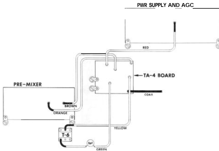
TA-4 PICTORIAL WIRING DIAGRAM (c) R.L. DRAKE VIRTUAL MUSEUM
